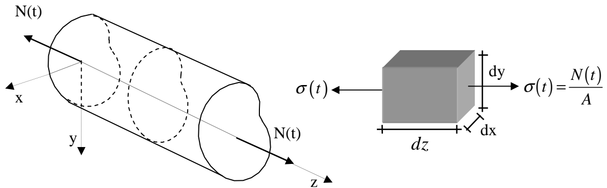
Figure 2. De Saint Venant visco-elastic bar in traction and an elementary volume
